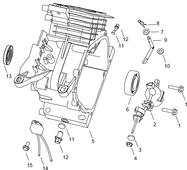
Cylinder barrel
